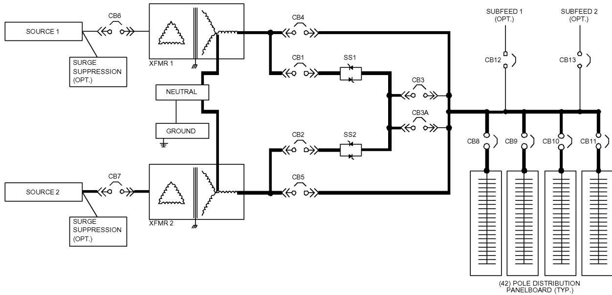
Figure 6 Typical Liebert STS2/PDU, one-line diagram, with I-Line distribution, dual static switch output circuit breakers
