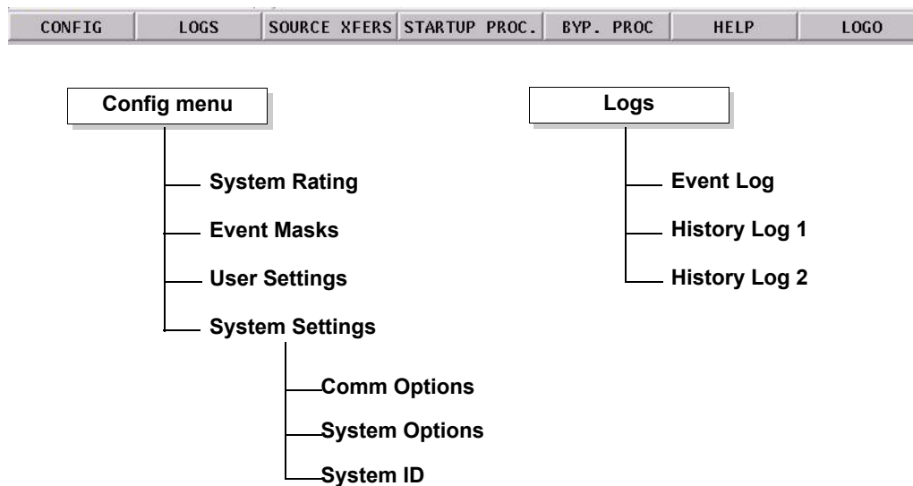
Figure 62 Menus
