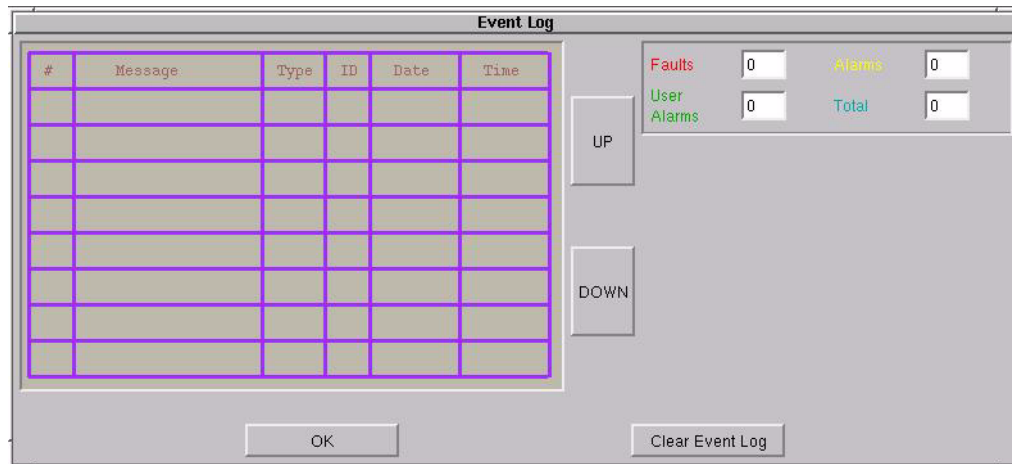
Figure 75 Event log
