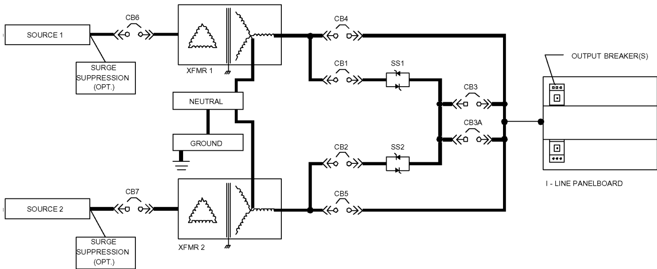
Figure 6 Typical Liebert STS2/PDU, one-line diagram, with I-Line distribution, dual static switch output circuit breakers
