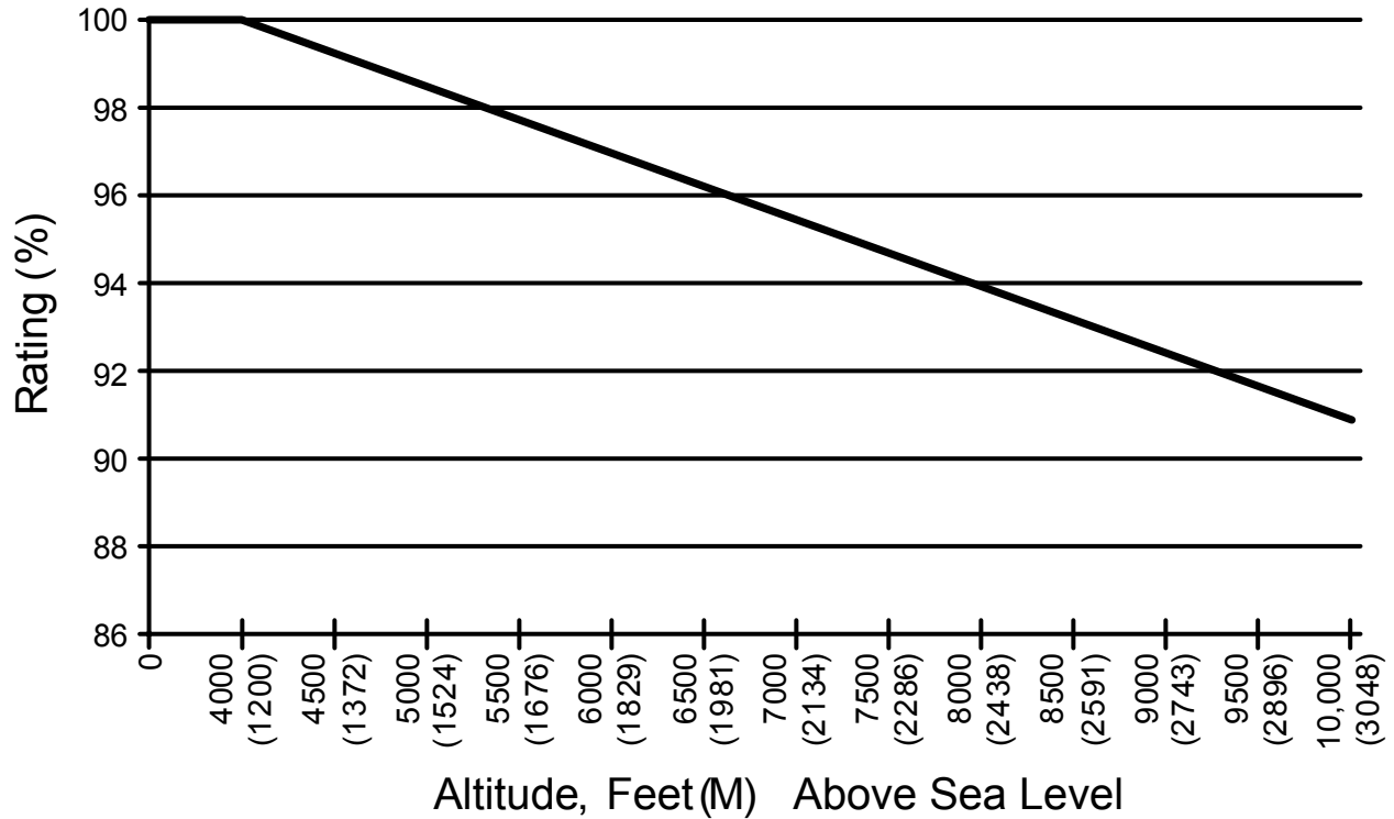
Figure 1 Recommended derating for high altitude operation
