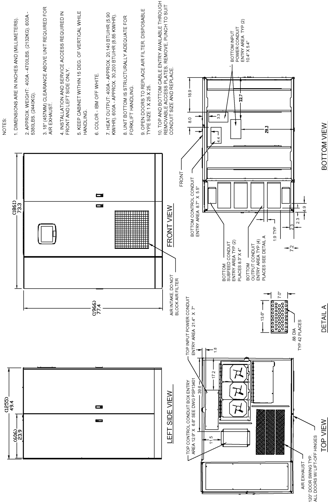
Figure 14 Outline drawing, 400-600A Liebert STS2/PDU with left side inline distribution
