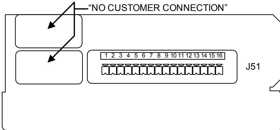
Figure 51 Control wiring for the input contact isolator board option
