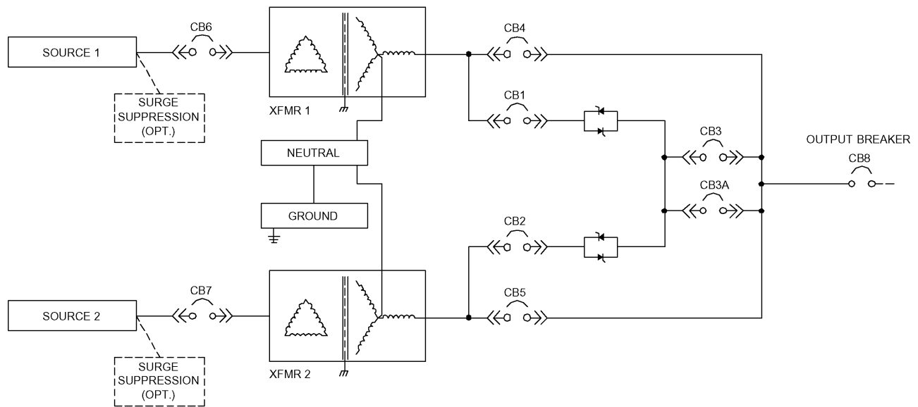
Figure 4 Typical Liebert STS2/PDU, one-line diagram, with dual static switch output circuit breakers (not available on 250A units)
