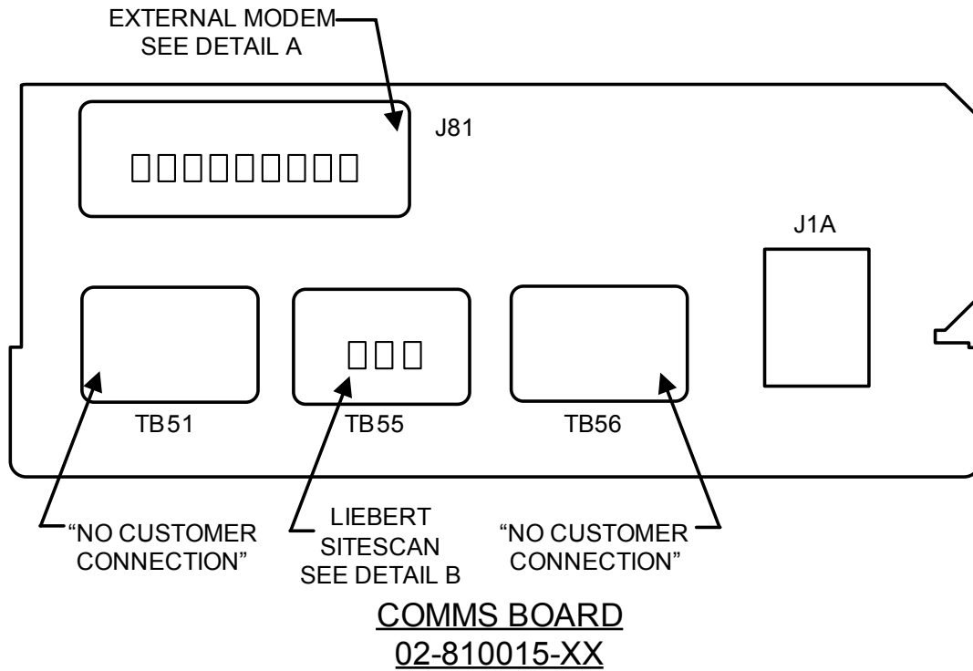
Figure 52 Control wiring for comms board
