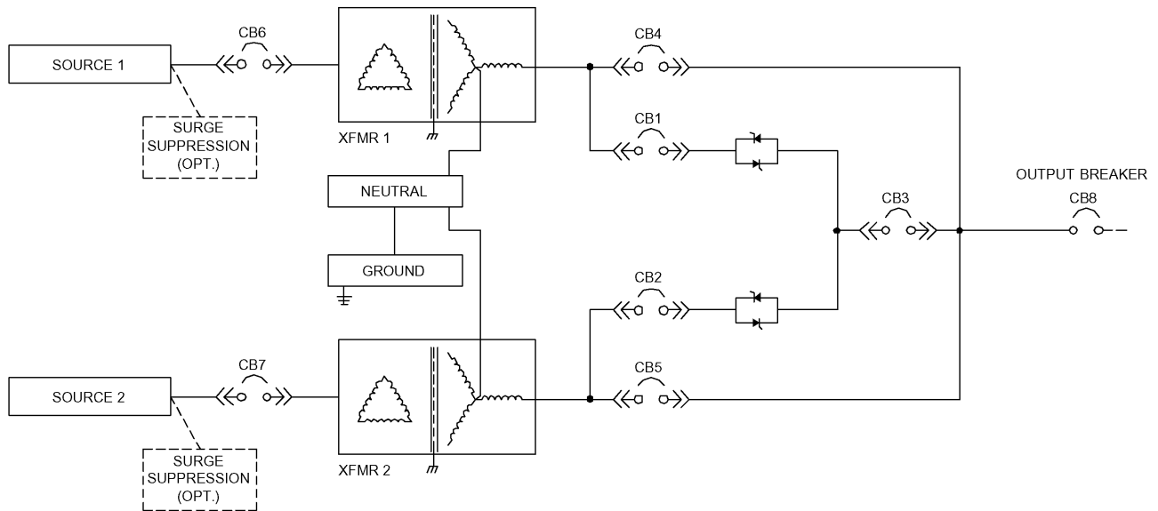
Figure 3 Typical Liebert STS2/PDU, one-line diagram
