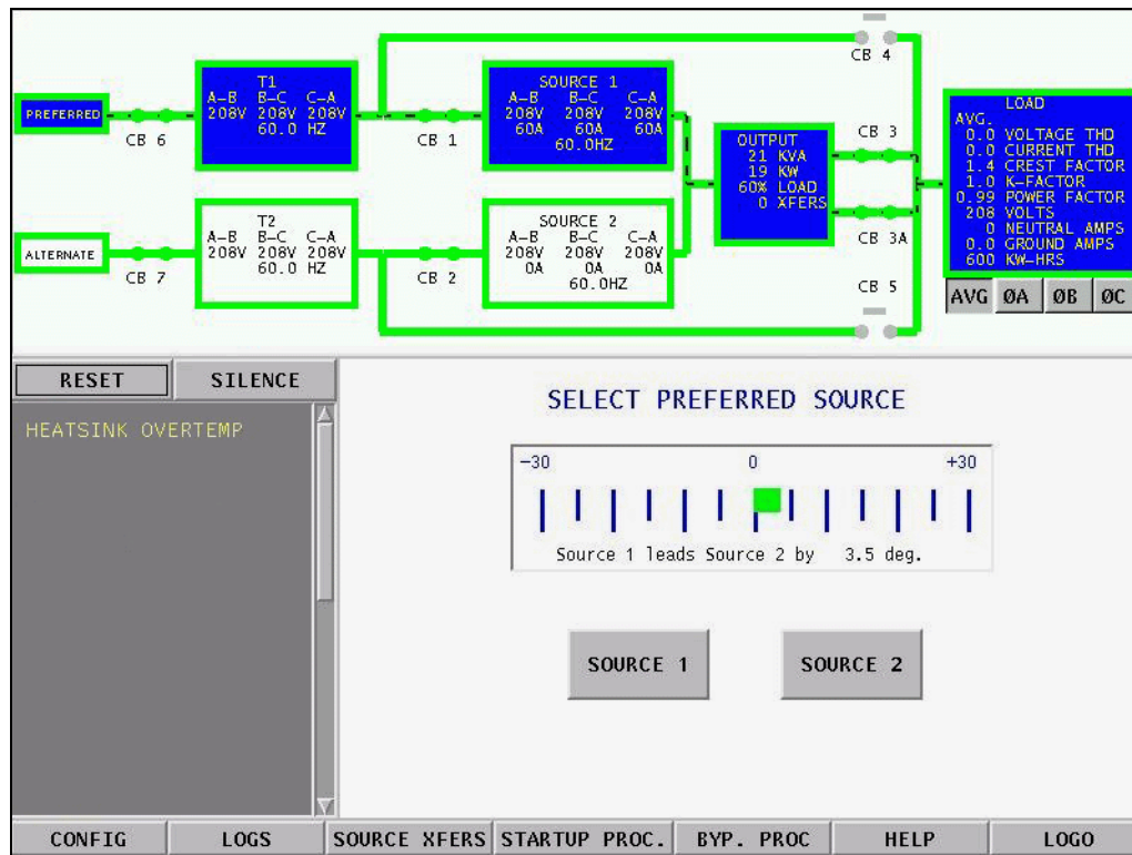
Figure 59 Source Transfer screen
