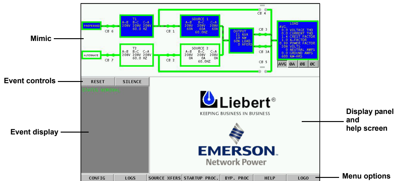
Figure 61 Liebert STS2/PDU Touch Screen Display
