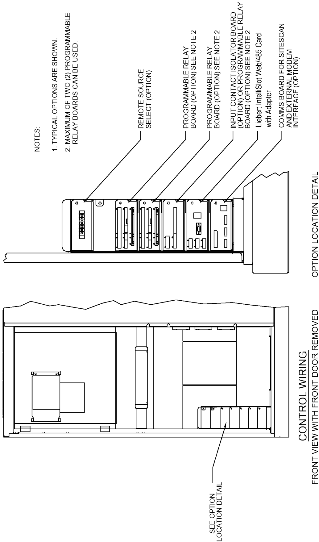
Figure 48 Control connection location, 400-800A Liebert STS2/PDU
