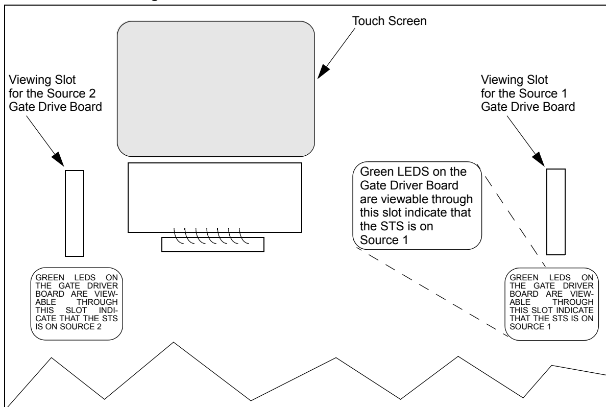
Figure 60 Gate board viewing slot locations
